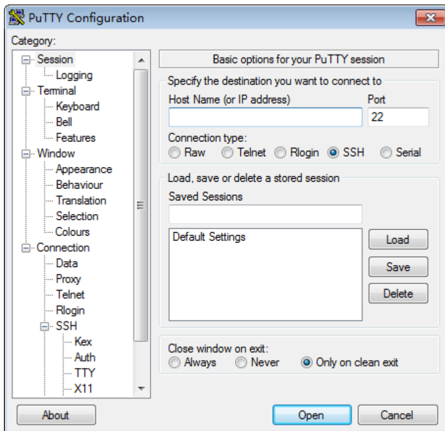
图 8-19 PuTTY Configuration
